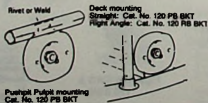
Typical mounting for Cruiser Masthead Lantern Cat. No. 120 RB BKT
