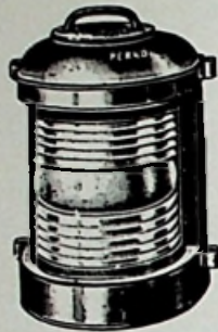
Fig. 1002 Masthead or Range Light 225 Degrees
