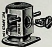
Rear view showing method of changing bulb
